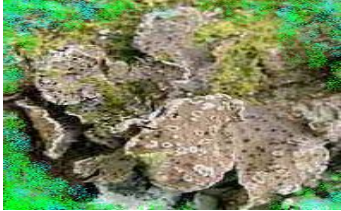
Lobariascrobiculata
